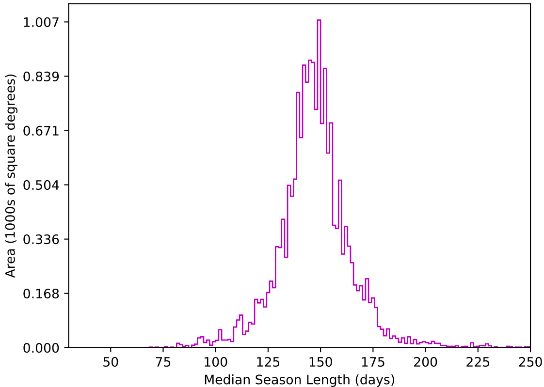
ddf_acor_sf10_lsf20_lsr20_v3.4_10yrs WFD z band: Median Season Length
