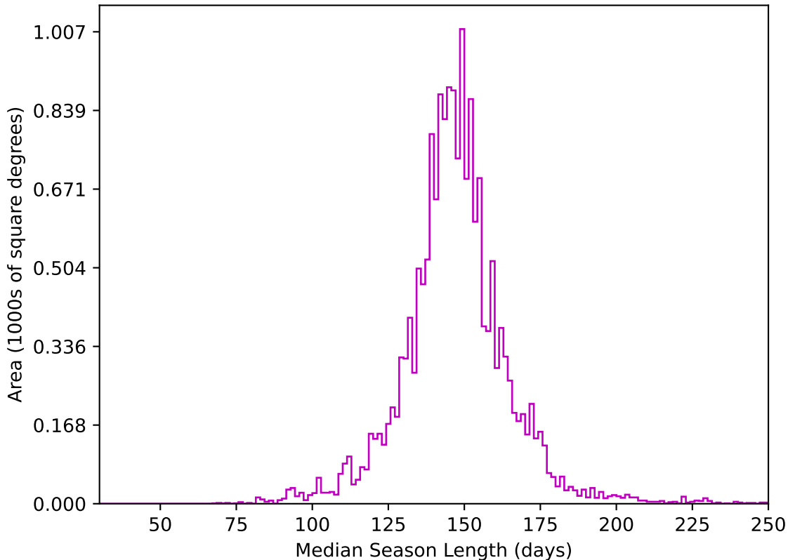
ddf_acor_sf10_lsf20_lsr20_v3.4_10yrs WFD z band: Median Season Length
