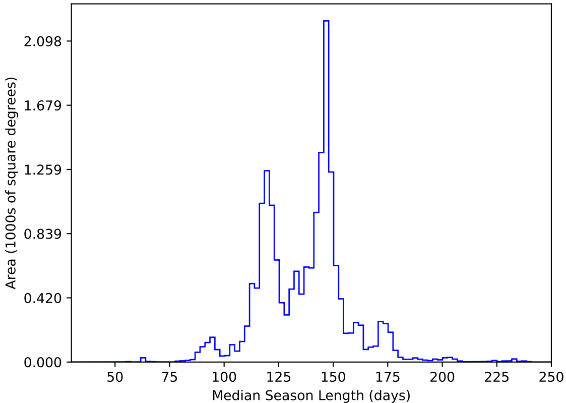
ddf_acor_sf10_lsf20_lsr20_v3.4_10yrs WFD y band: Median Season Length
