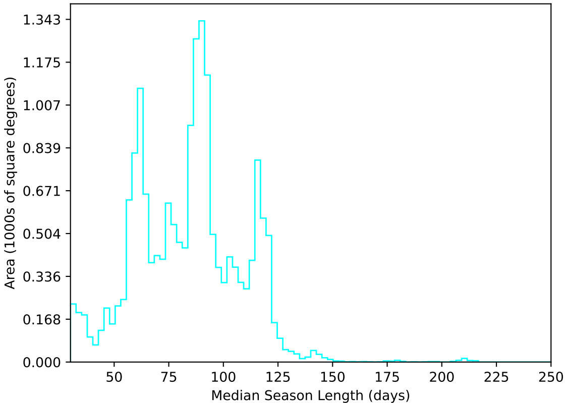
ddf_acor_sf10_ls20_lsr20_v3.4_10yrs WFD u band: Median Season Length
