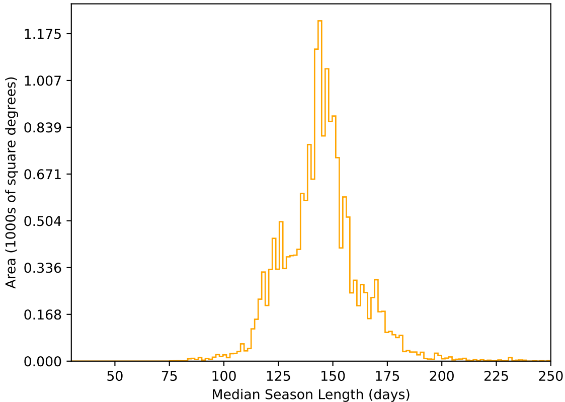
ddf_acor_sf10_lsf20_lsr20_v3.4_10yrs WFD r band: Median Season Length
