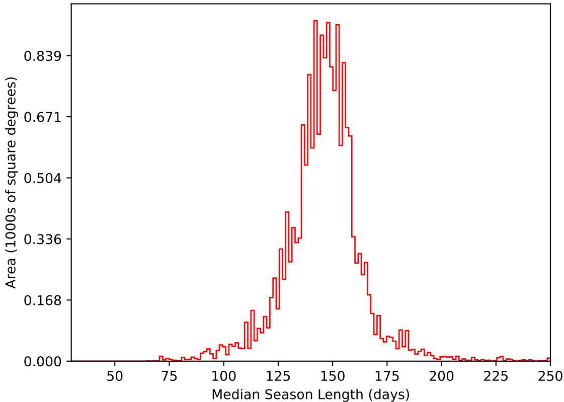
ddf_acor_sf10_lsf20_lsr20_v3.4_10yrs WFD i band: Median Season Length
