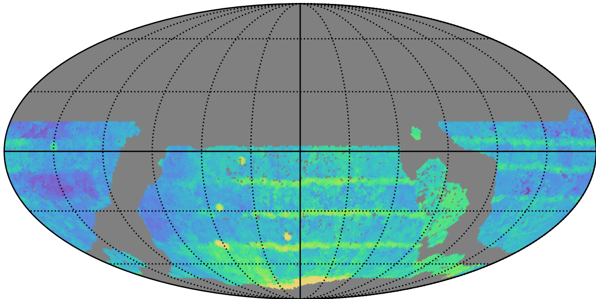
ddf_acor_sf10_lsf20_lsr20_v3.4_10yrs WFD all bands: Median Season Length
