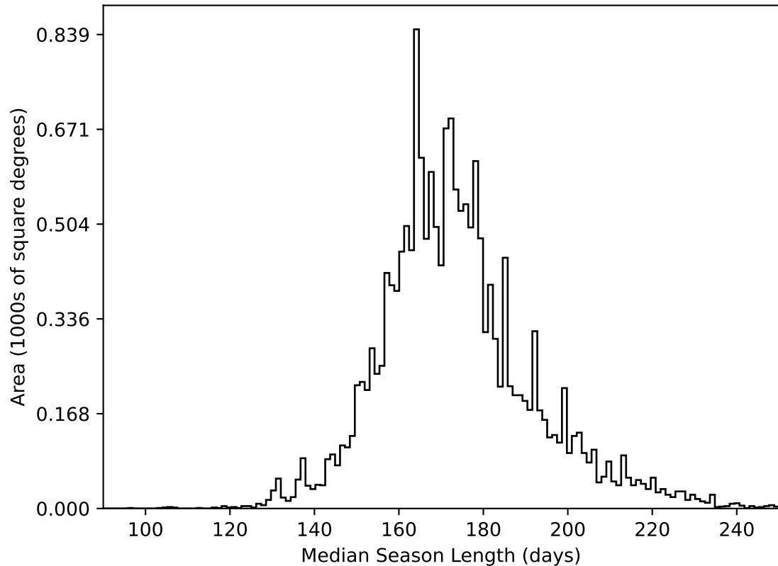
ddf_acor_sf10_lsf20_lsr20_v3.4_10yrs WFD all bands: Median Season Length
