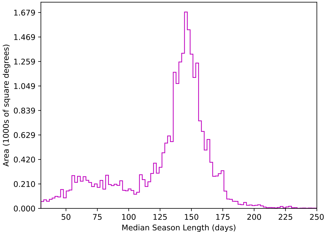
ddf_acor_sf10_lsf20_lsr20_v3.4_10yrs All sky z band: Median Season Length
