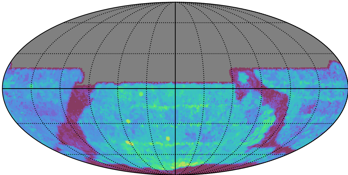
ddf_acor_sf10_lsf20_lsr20_v3.4_10yrs All sky y band: Median Season Length
