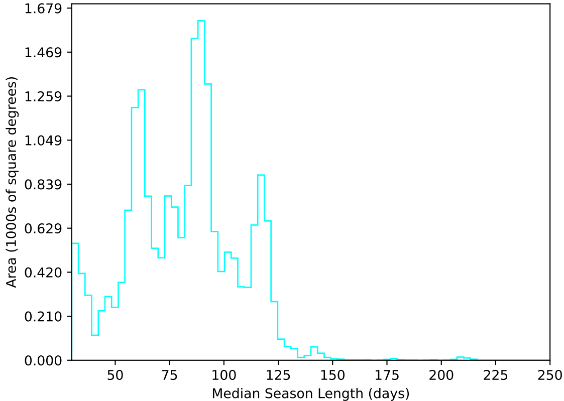
ddf_acor_sf10_lsf20_lsr20_v3.4_10yrs All sky u band: Median Season Length
