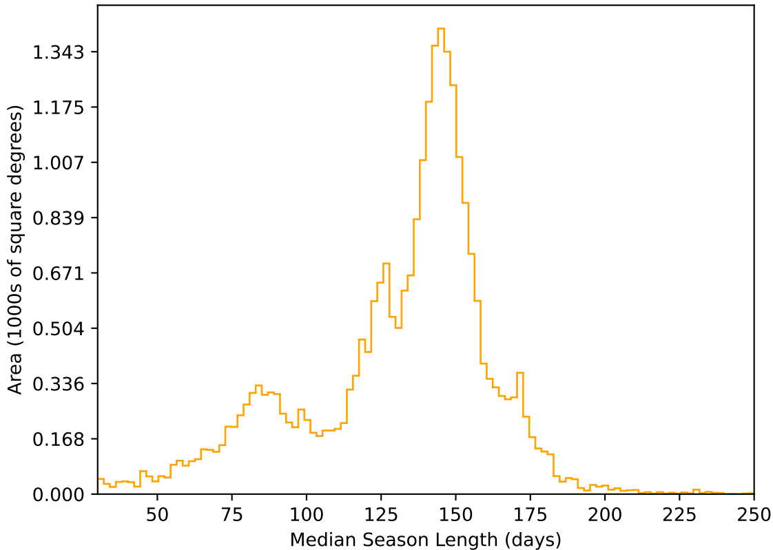
ddf_acor_sf10_lsf20_lsr20_v3.4_10yrs All sky r band: Median Season Length
