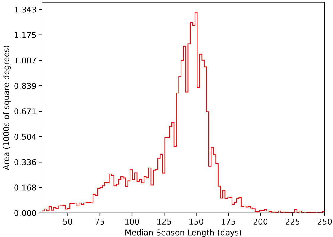
ddf_acor_sf10_lsf20_lsr20_v3.4_10yrs All sky i band: Median Season Length
