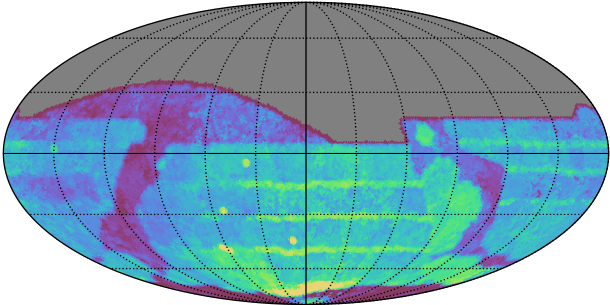
ddf_acor_sf10_lsf20_lsr20_v3.4_10yrs All sky all bands: Median Season Length
