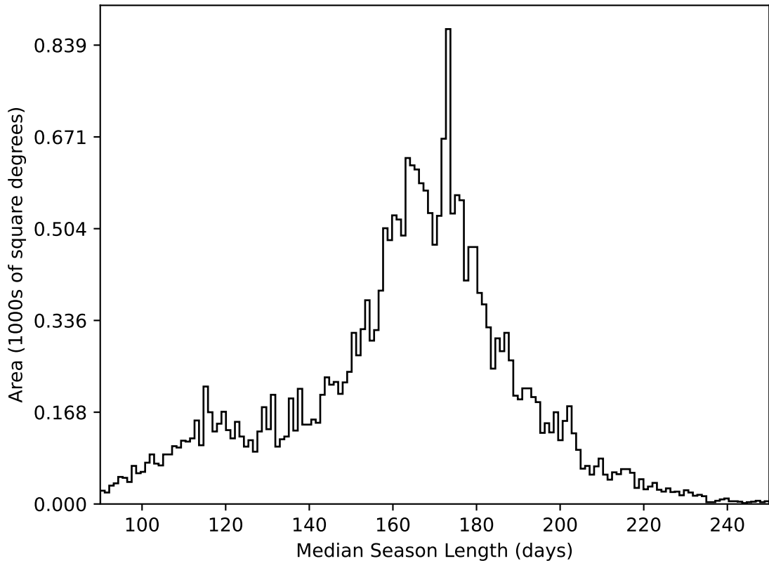
ddf_acor_sf10_lsf20_lsr20_v3.4_10yrs All sky all bands: Median Season Length
