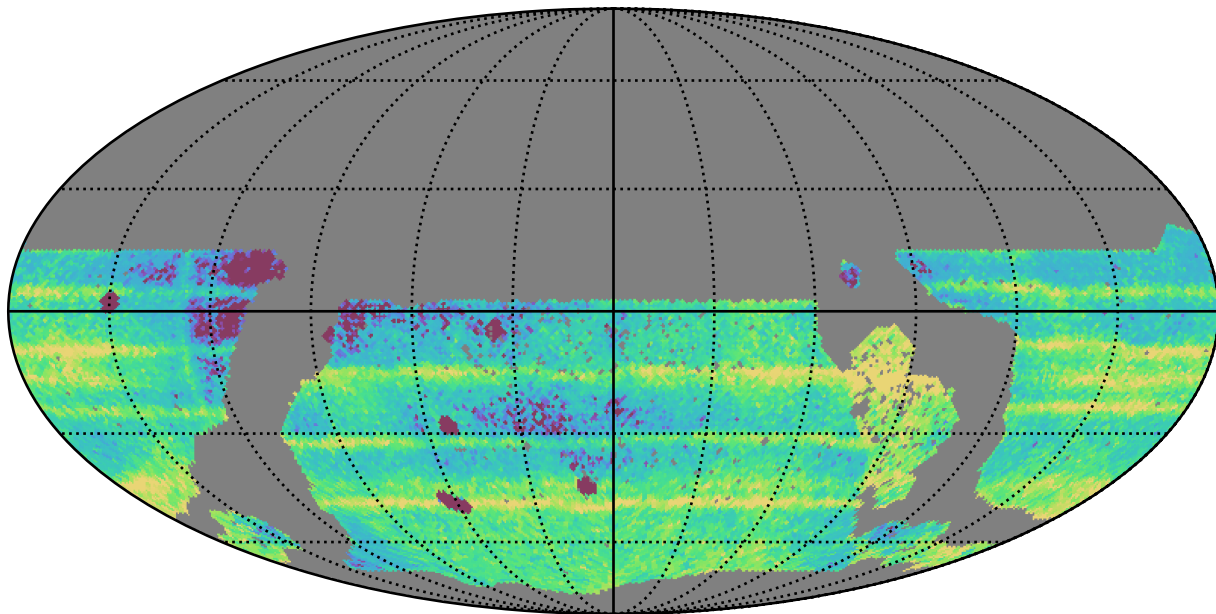
ddf_acor_sf10_lsf20_lsr20_v3.4_10yrs WFD: Median Intra-Night Gap
