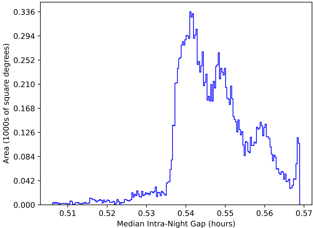
ddf_acor_sf10_lsf20_lsr20_v3.4_10yrs WFD: Median Intra-Night Gap
