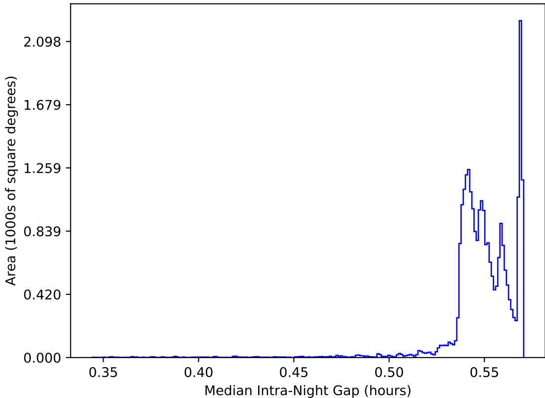
ddf_acor_sf10_lsf20_lsr20_v3.4_10yrs All sky: Median Intra-Night Gap
