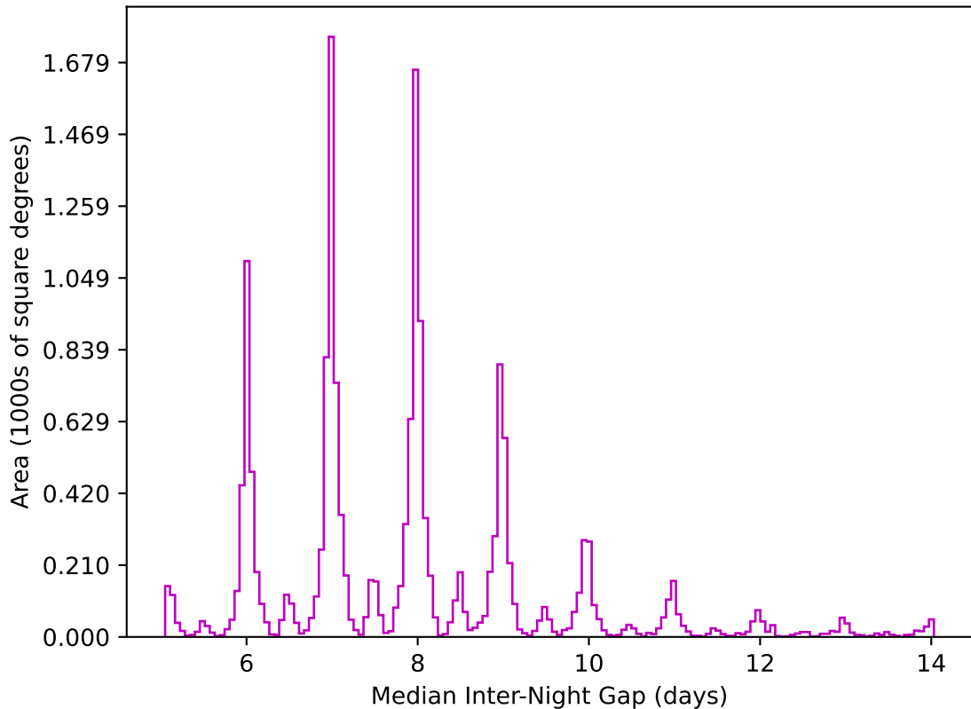
ddf_acor_sf10_lsf20_lsr20_v3.4_10yrs WFD z band: Median Inter-Night Gap
