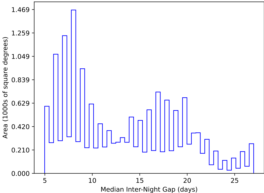
ddf_acor_sf10_lsf20_lsr20_v3.4_10yrs WFD y band: Median Inter-Night Gap
