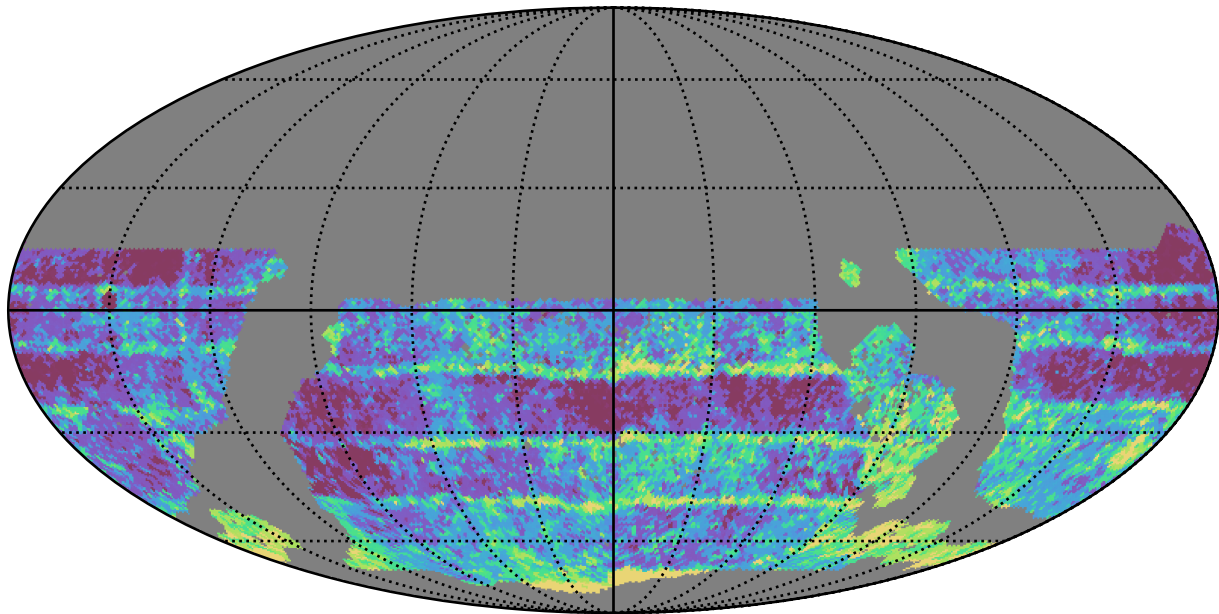
ddf_acor_sf10_lsf20_lsr20_v3.4_10yrs WFD r band: Median Inter-Night Gap
