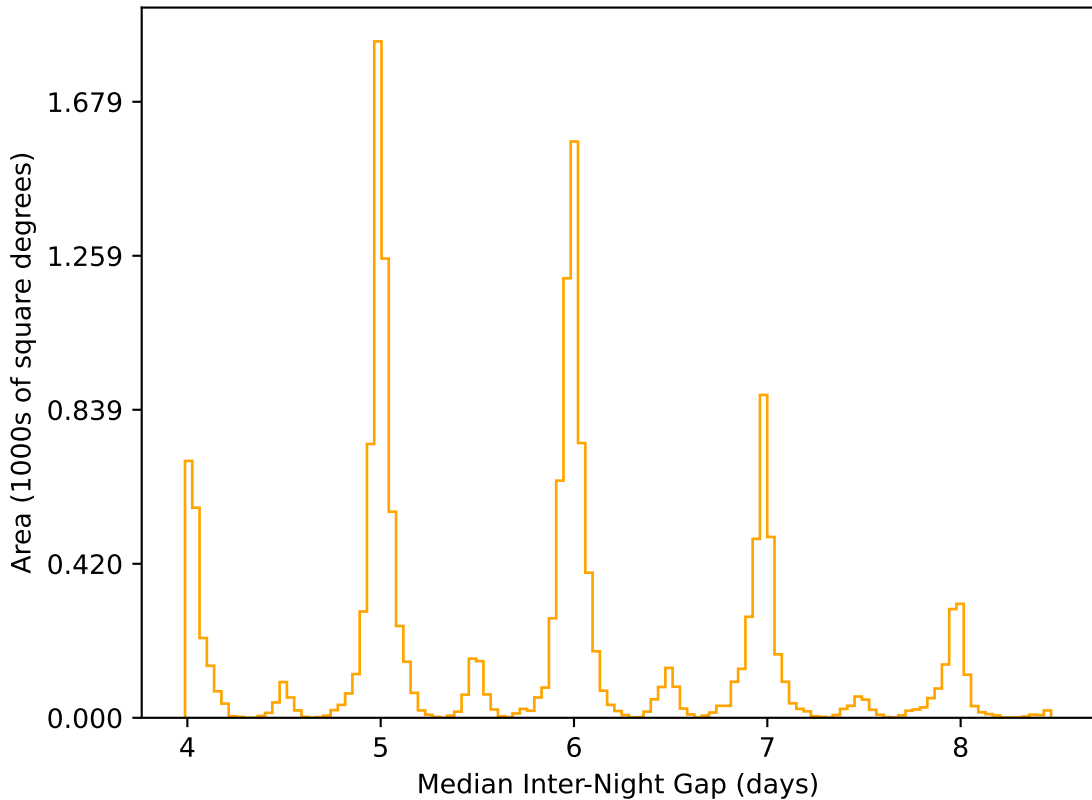
ddf_acor_sf10_lsf20_lsr20_v3.4_10yrs WFD r band: Median Inter-Night Gap
