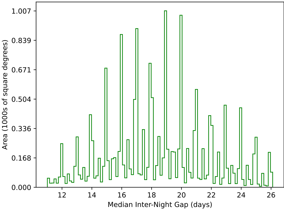
ddf_acor_sf10_lsf20_lsr20_v3.4_10yrs WFD g band: Median Inter-Night Gap
