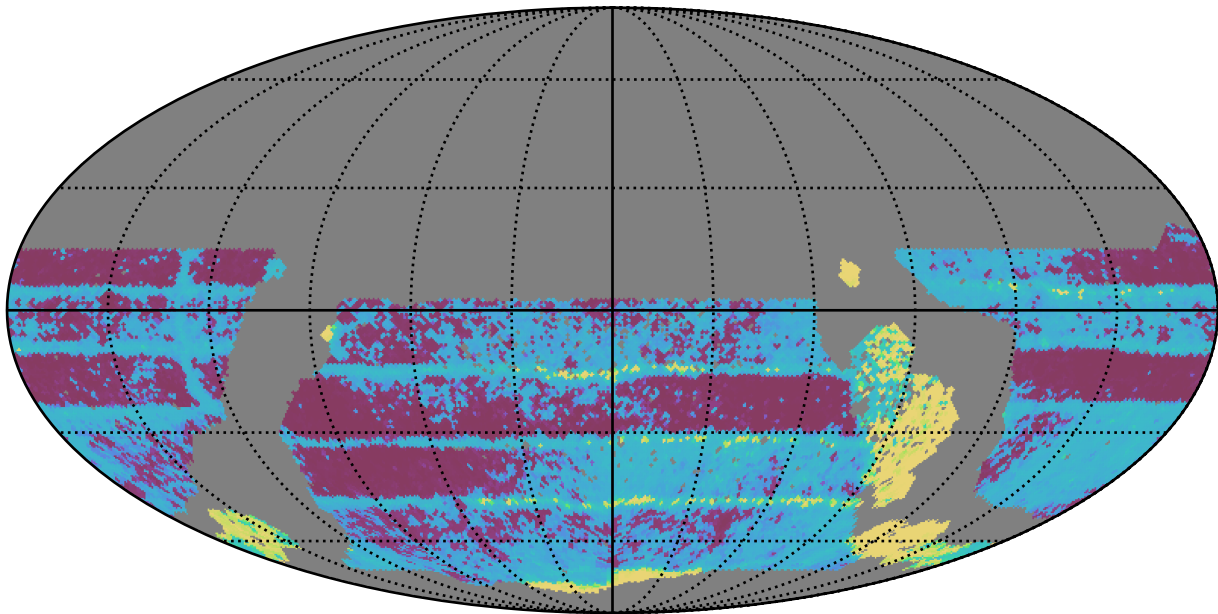
ddf_acor_sf10_lsf20_lsr20_v3.4_10yrs WFD all bands: Median Inter-Night Gap
