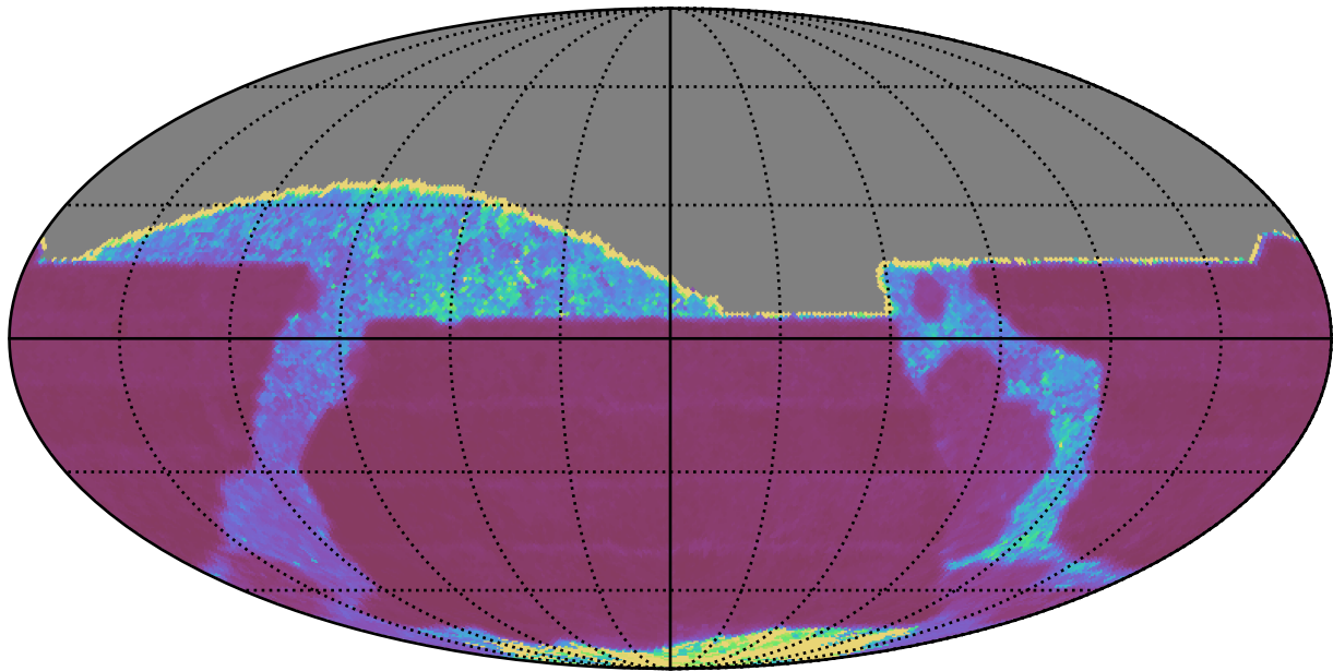
ddf_acor_sf10_lsf20_lsr20_v3.4_10yrs All sky z band: Median Inter-Night Gap
