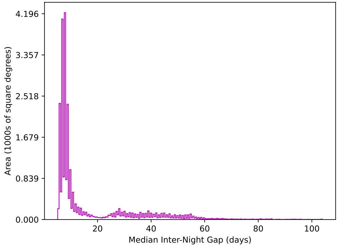
ddf_acor_sf10_lsf20_lsr20_v3.4_10yrs All sky z band: Median Inter-Night Gap
