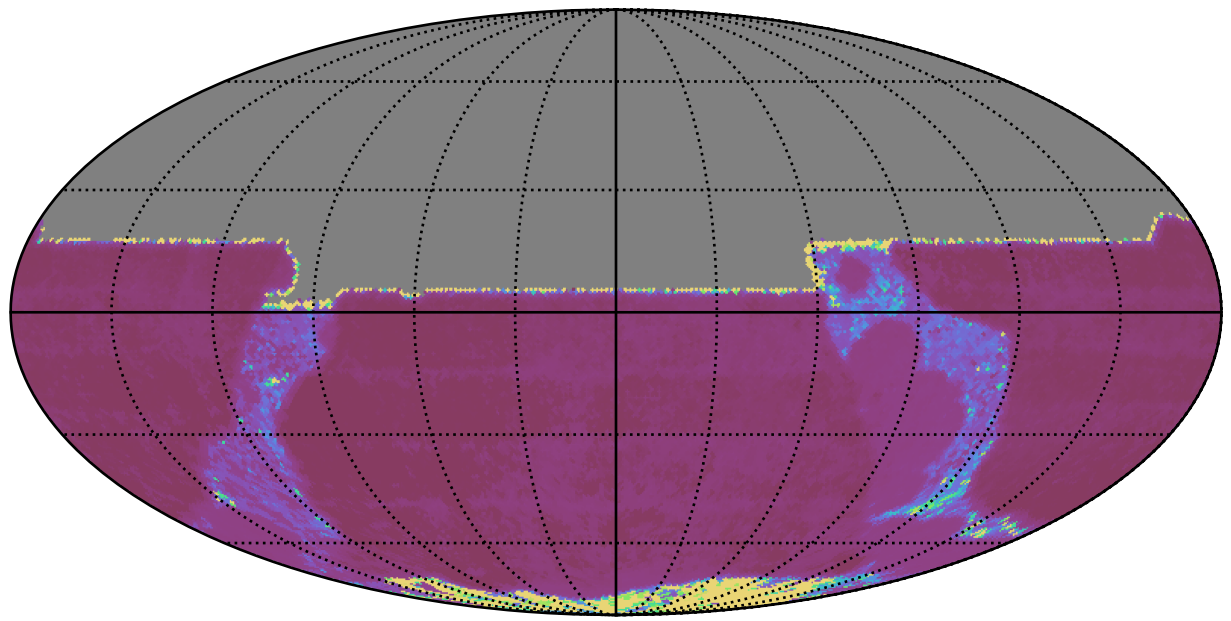
ddf_acor_sf10_lsf20_lsr20_v3.4_10yrs All sky y band: Median Inter-Night Gap
