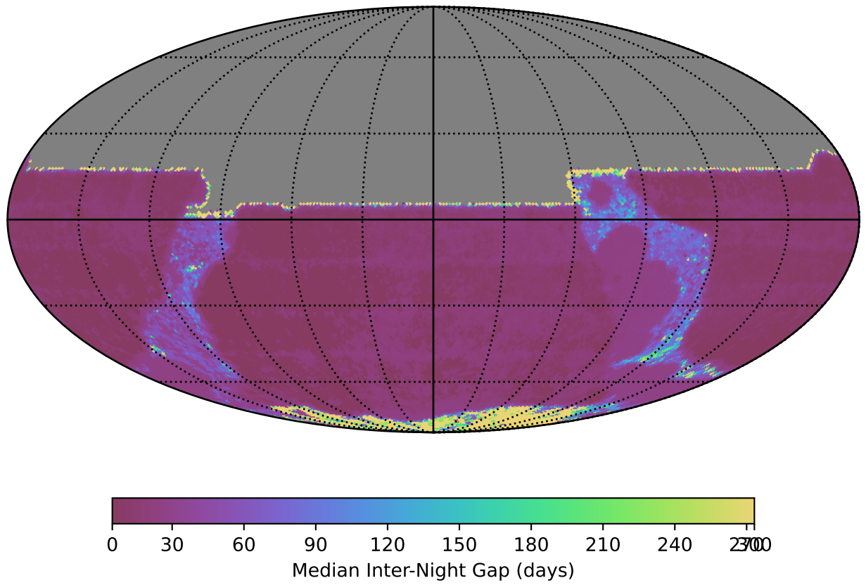
ddf_acor_sf10_lsf20_lsr20_v3.4_10yrs All sky y band: Median Inter-Night Gap
