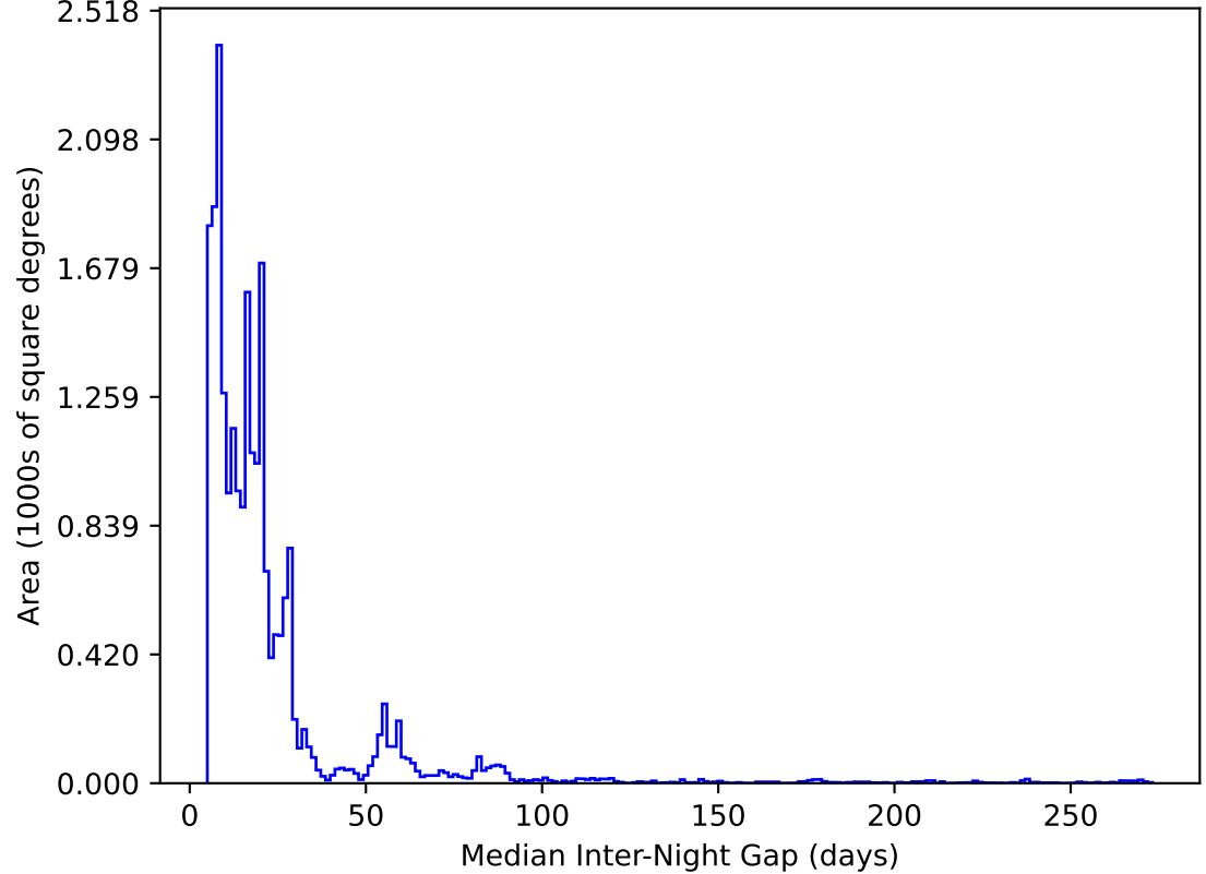
ddf_acor_sf10_lsf20_lsr20_v3.4_10yrs All sky y band: Median Inter-Night Gap
