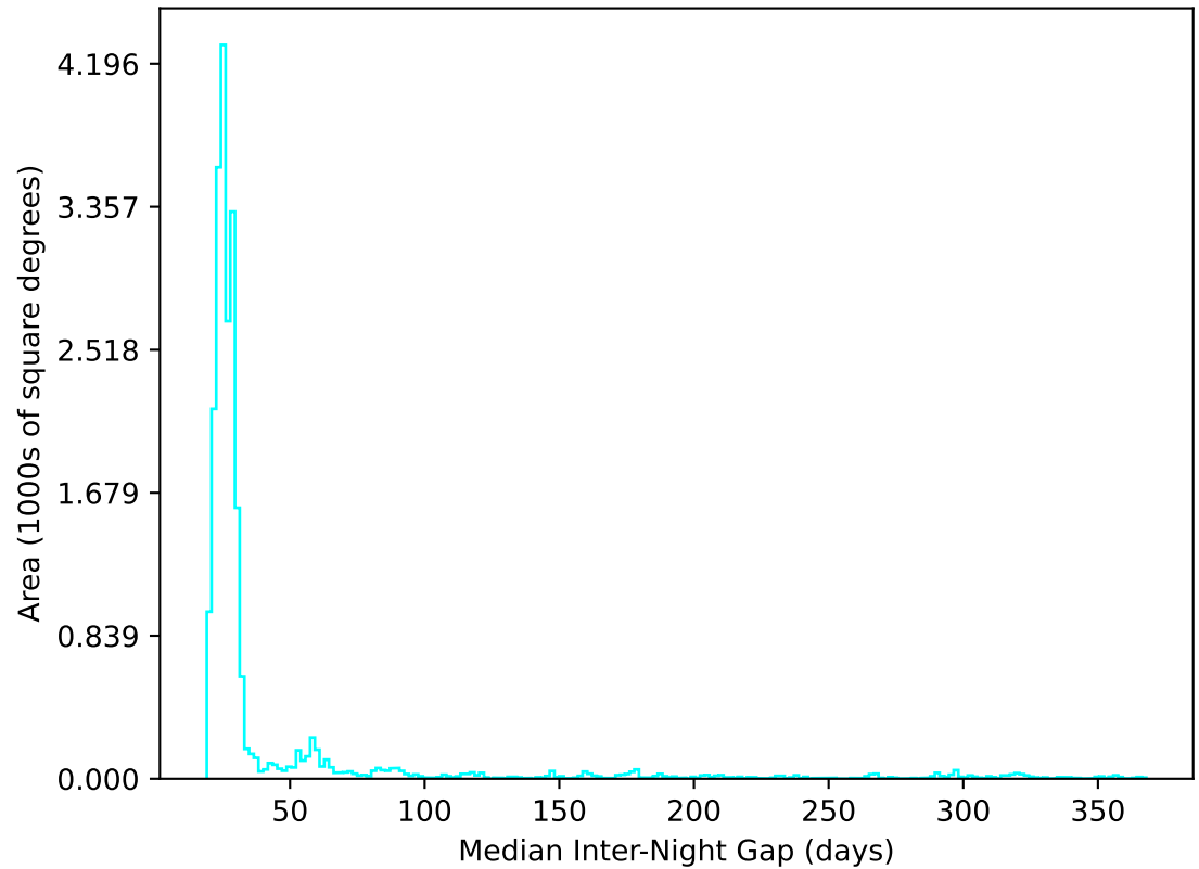
ddf_acor_sf10_lsf20_lsr20_v3.4_10yrs All sky u band: Median Inter-Night Gap
