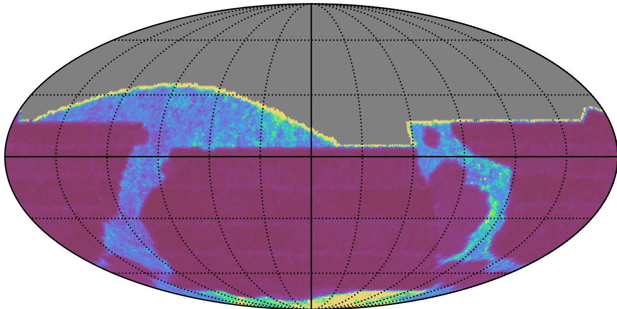
ddf_acor_sf10_lsf20_lsr20_v3.4_10yrs All sky i band: Median Inter-Night Gap
