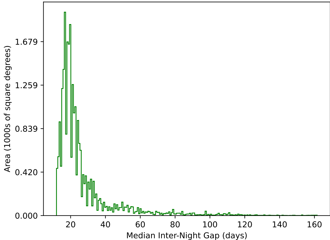
ddf_acor_sf10_lsf20_lsr20_v3.4_10yrs All sky g band: Median Inter-Night Gap
