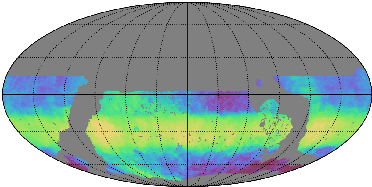
ddf_acor_sf10_lsf20_lsr20_v3.4_10yrs WFD z band: Median HA
