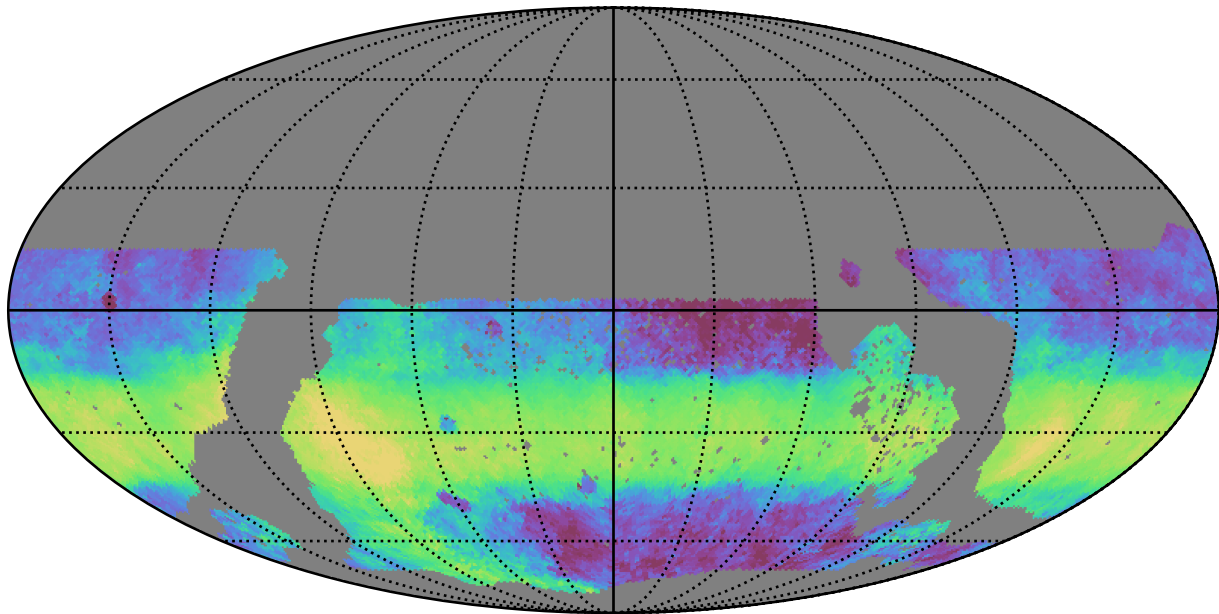
ddf_acor_sf10_lsf20_lsr20_v3.4_10yrs WFD y band: Median HA
