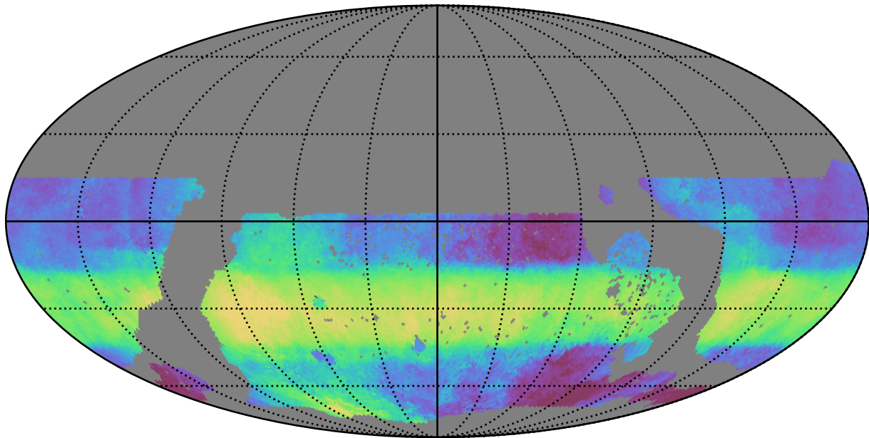
ddf_acor_sf10_lsf20_lsr20_v3.4_10yrs WFD r band: Median HA
