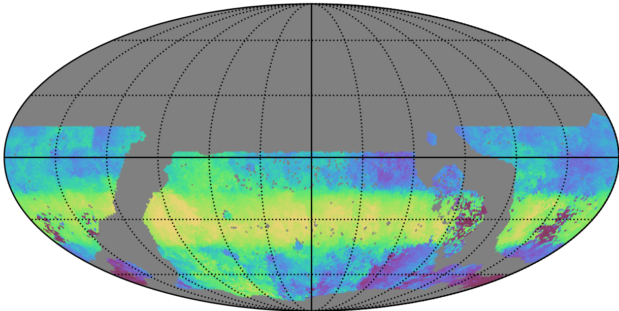
ddf_acor_sf10_lsf20_lsr20_v3.4_10yrs WFD g band: Median HA
