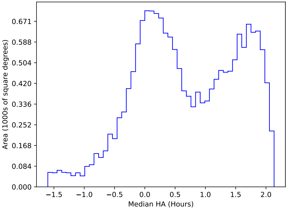
ddf_acor_sf10_lsf20_lsr20_v3.4_10yrs WFD g band: Median HA
