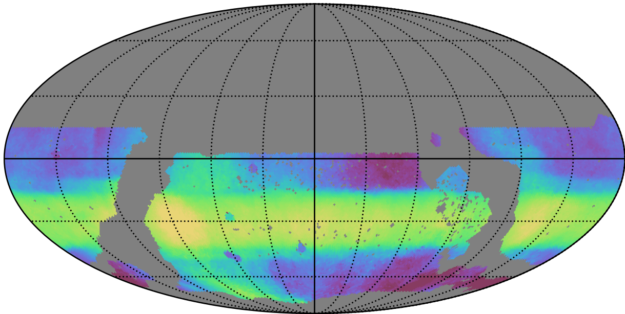
ddf_acor_sf10_lsf20_lsr20_v3.4_10yrs WFD all bands: Median HA
