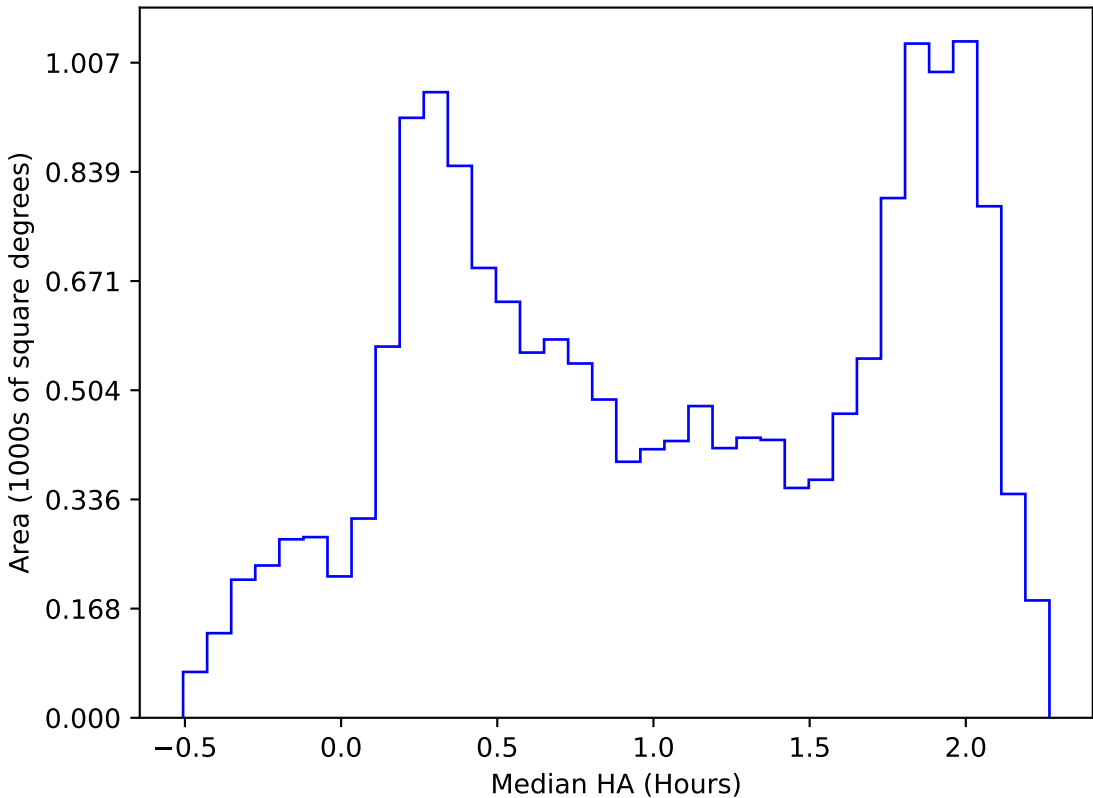
ddf_acor_sf10_lsf20_lsr20_v3.4_10yrs WFD all bands: Median HA
