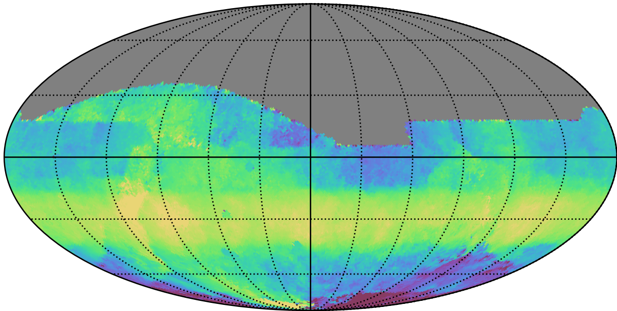
ddf_acor_sf10_lsf20_lsr20_v3.4_10yrs All sky z band: Median HA
