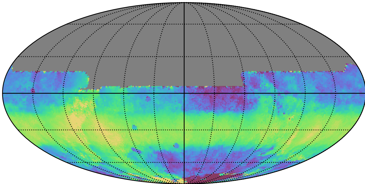
ddf_acor_sf10_lsf20_lsr20_v3.4_10yrs All sky y band: Median HA
