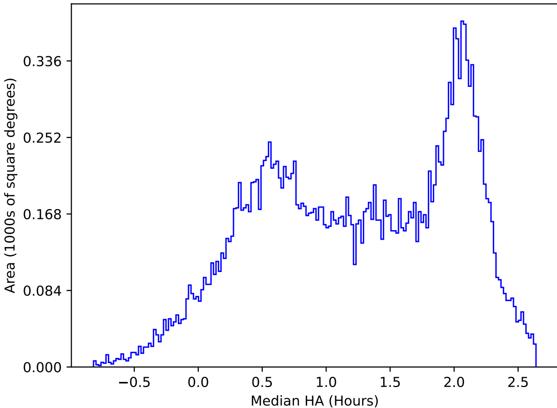
ddf_acor_sf10_lsf20_lsr20_v3.4_10yrs All sky y band: Median HA
