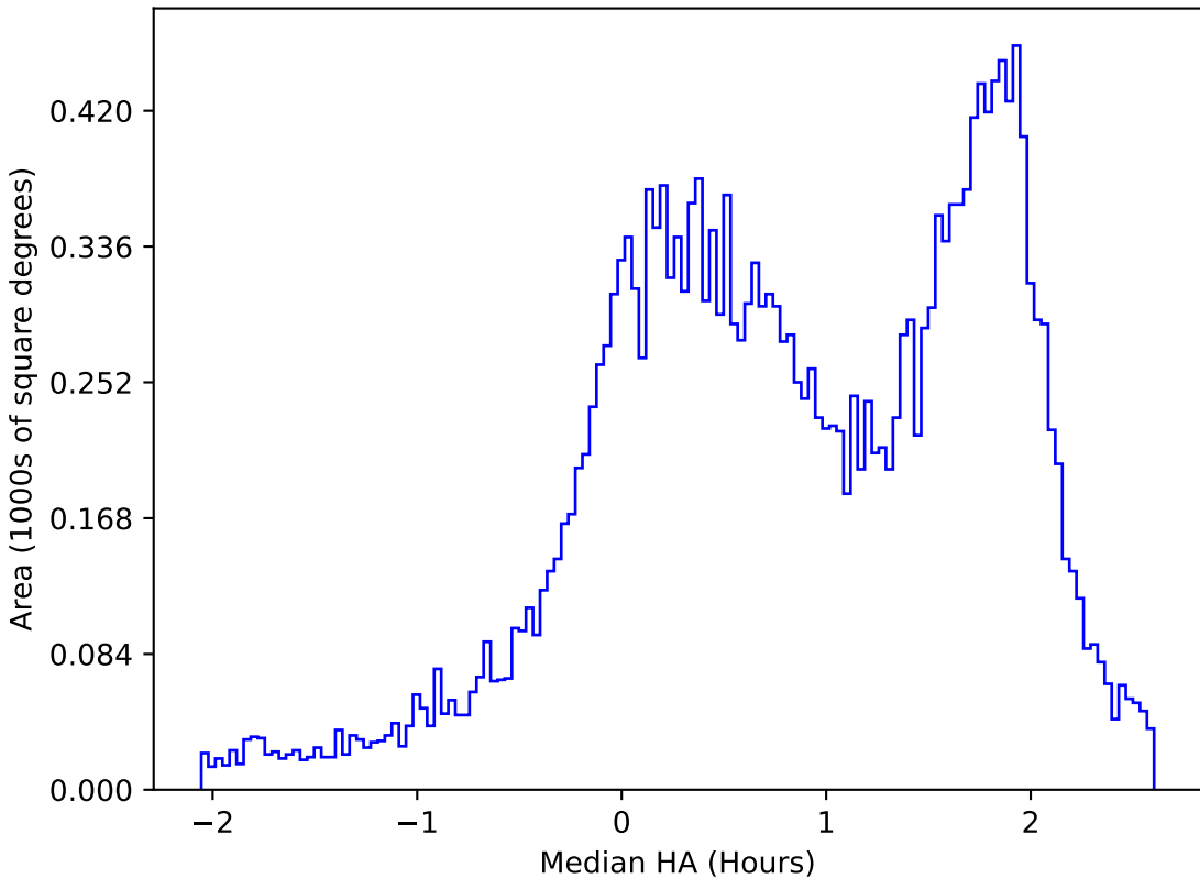
ddf_acor_sf10_ls20_lsr20_v3.4_10yrs All sky u band: Median HA
