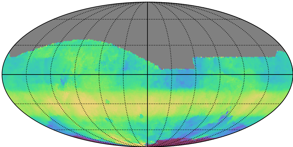
ddf_acor_sf10_lsf20_lsr20_v3.4_10yrs All sky r band: Median HA
