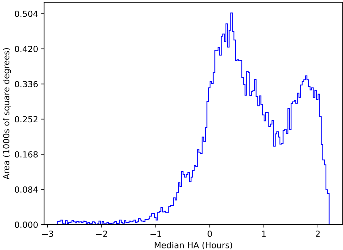
ddf_acor_sf10_lsf20_lsr20_v3.4_10yrs All sky r band: Median HA
