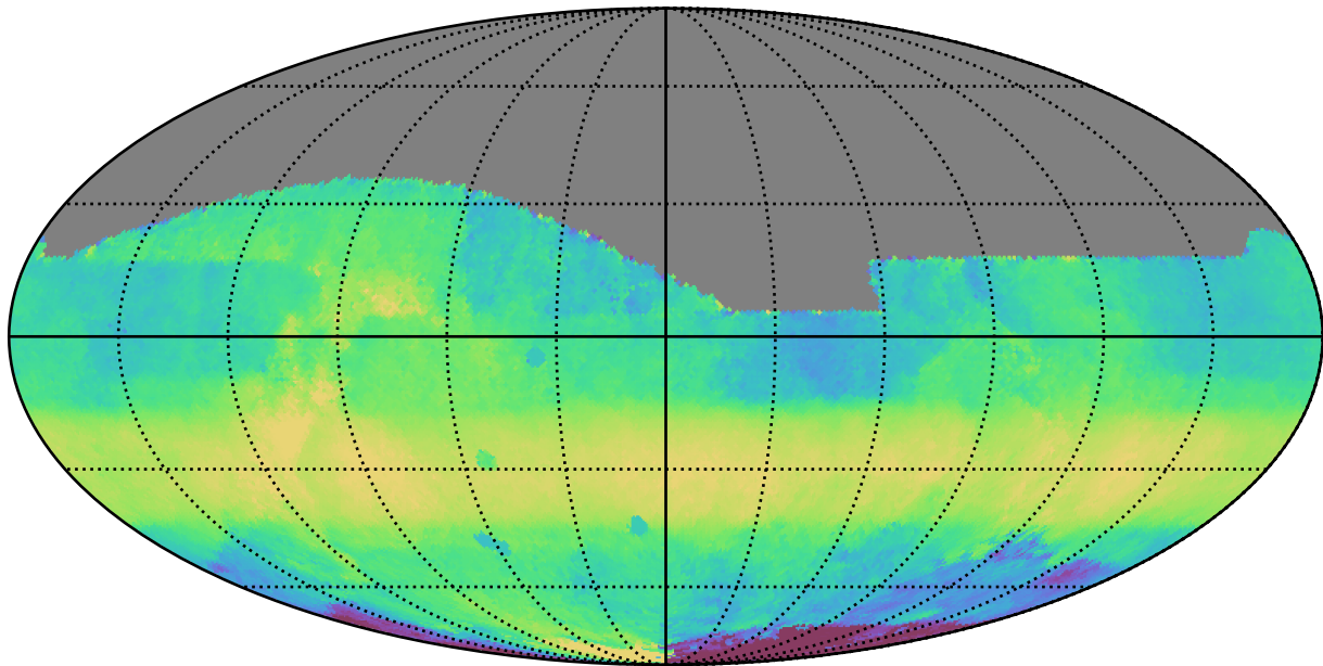
ddf_acor_sf10_lsf20_lsr20_v3.4_10yrs All sky i band: Median HA
