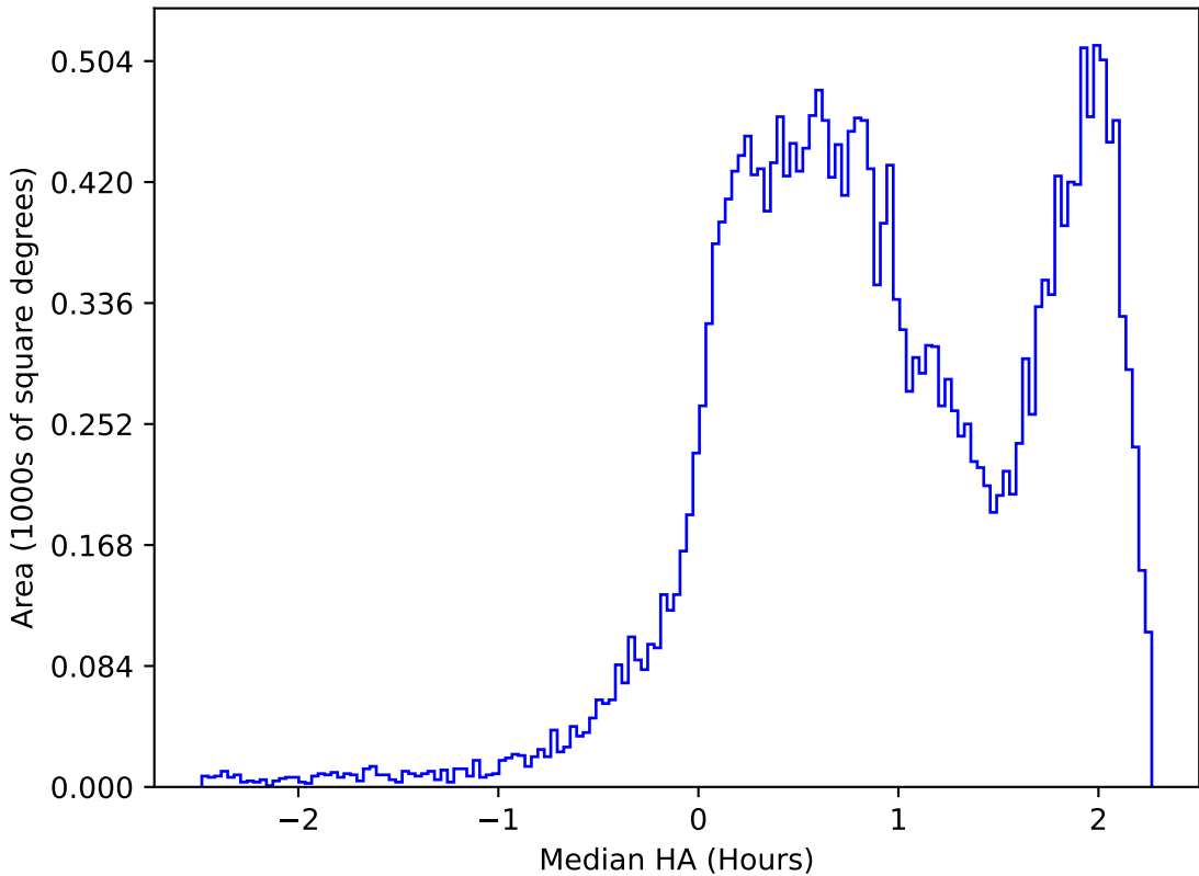
ddf_acor_sf10_lsf20_lsr20_v3.4_10yrs All sky i band: Median HA
