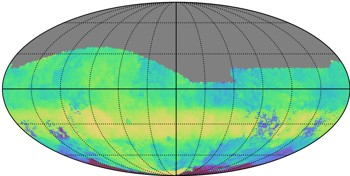
ddf_acor_sf10_lsf20_lsr20_v3.4_10yrs All sky g band: Median HA
