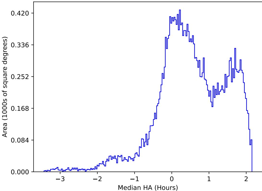
ddf_acor_sf10_ls20_lsr20_v3.4_10yrs All sky g band: Median HA
