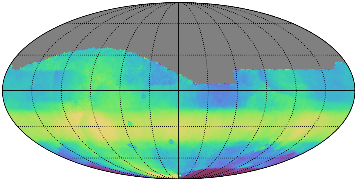
ddf_acor_sf10_lsf20_lsr20_v3.4_10yrs All sky all bands: Median HA
