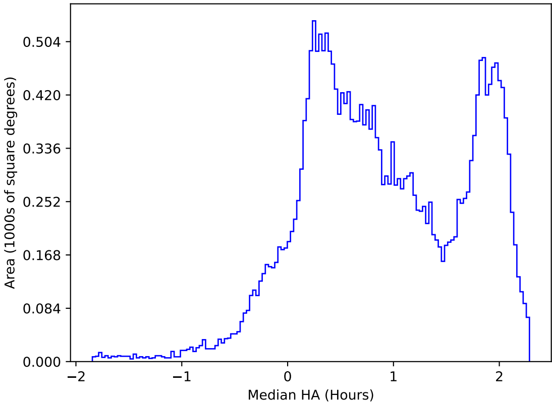
ddf_acor_sf10_lsf20_lsr20_v3.4_10yrs All sky all bands: Median HA
