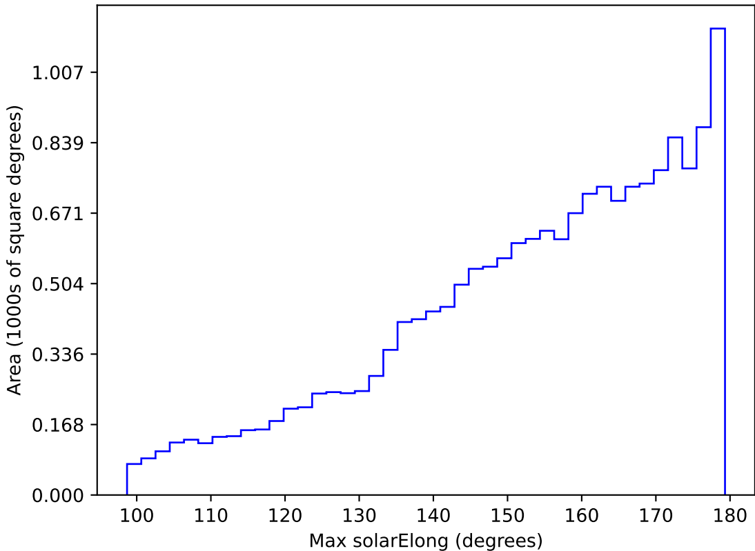
ddf_acor_sf10_lsf20_lsr20_v3.4_10yrs WFD z band: Max solarElong
